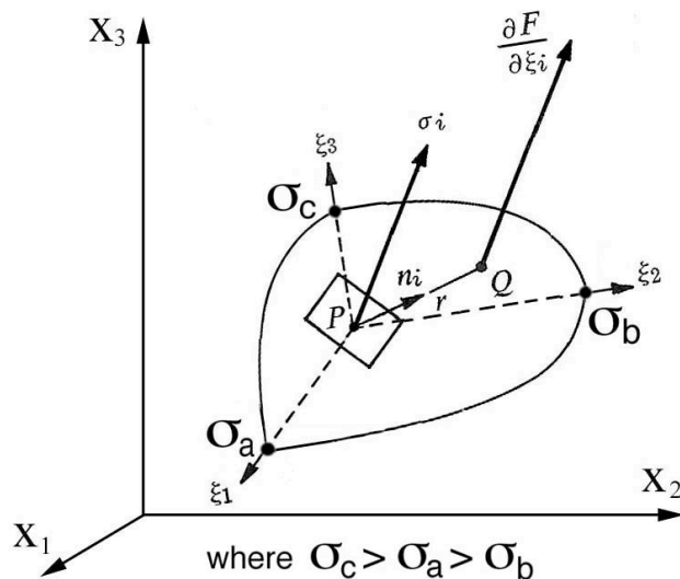
Figure 2: Stress quadric surface at P is aligned along the principal axes, \xi_i , and shows only a portion of the ellipsoid.
