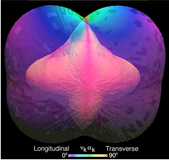
Figure 7: Combined wave velocity surface for Calcium-Formate where translucent outer surfaces show a single connected surface, C_{ijkl} [Ledbetter and Kriz (1992)].
