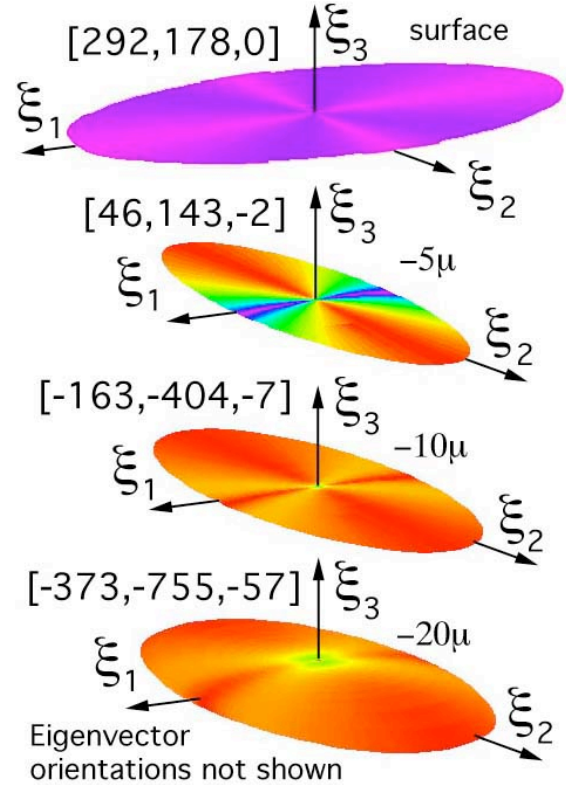
Figure 3b: Second order stress tensors plotted as stress ellipsoids at and below the surface for a material in a state of residual stress, where principal stresses are listed in brackets and aligned for comparison with depth, [Harting, (1998)].
