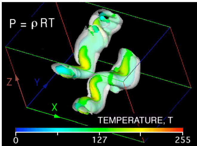
Figure 14: Extracting a linear zeroth order tensor equation from numerical data of a simulation where mixing occurs in a
