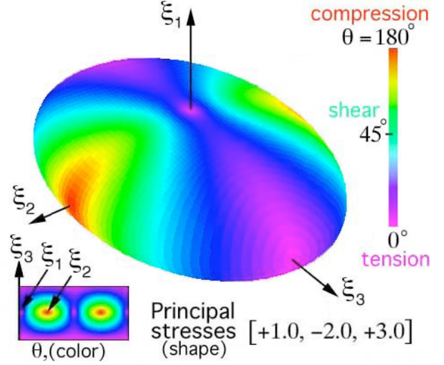
Figure 3a: Color map of normal-tension, shear, and normal-compressive stresses plotted on a stress ellipsoid surface.
