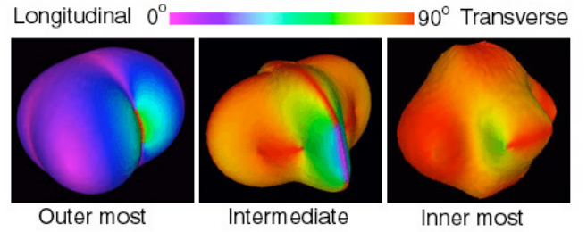
Figure 6: Wave velocity (eigenvalue) surfaces for Calcium-Formate, where color is the wave-type which is defined by the cosine of the angle, \hat{\rho}_k \hat{l}_k , separating two unit vectors: the vibration direction (eigenvector), \hat{\rho}_k , with respect to the propagation direction, \hat{l}_k .
