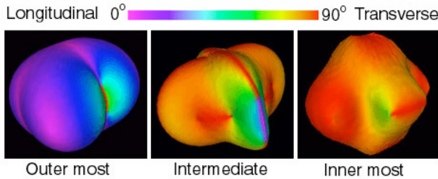
Figure 6: Wave velocity (eigenvalue) surfaces for Calcium-Formate, where color is the wave-type which is defined by the cosine of the angle, \square_k \square_k , separating two unit vectors: the vibration direction (eigenvector), \square_k , with respect to the propagation direction, \square_k .
