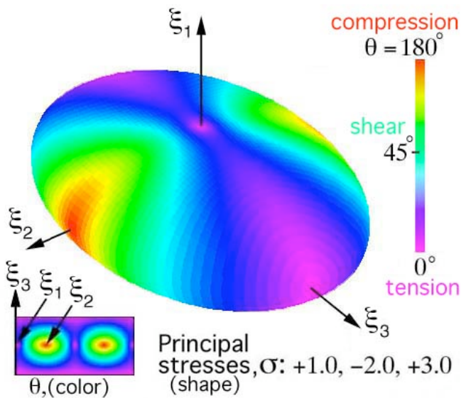
Figure 3: Color map of normal-tension, shear, and normal-compressive stresses plotted on a stress ellipsoid surface.
